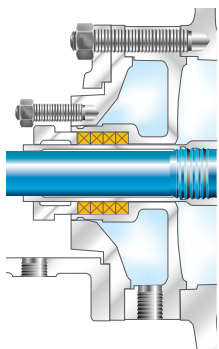
Cooled stuffing box
